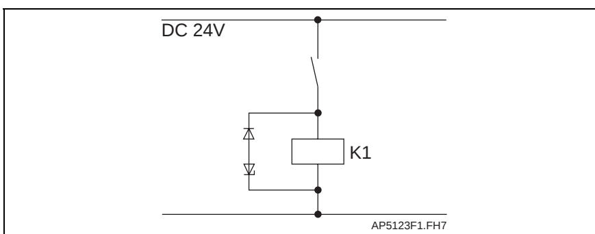
Fig. 6-20: Recommended protective circuits
