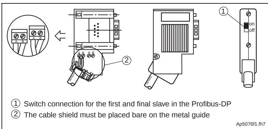
Fig. 5-73: Bus connection for the first and last slave without 9-pin D-SUB socket, INS 0540
