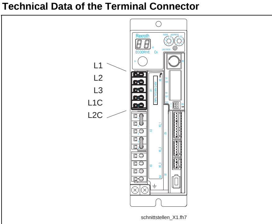
Fig. 5-6: Terminal connector X1
