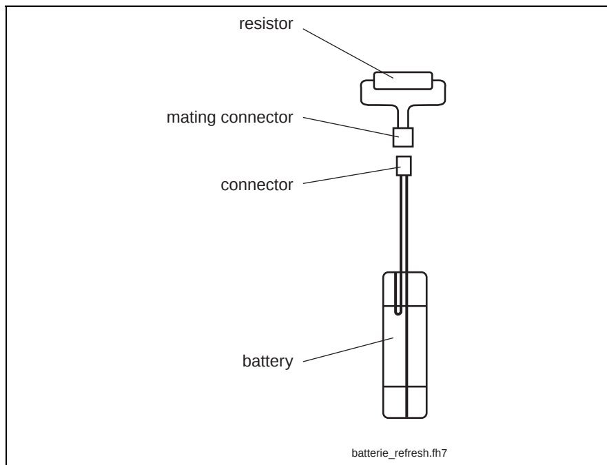
Fig. 8-55: Battery refreshing
